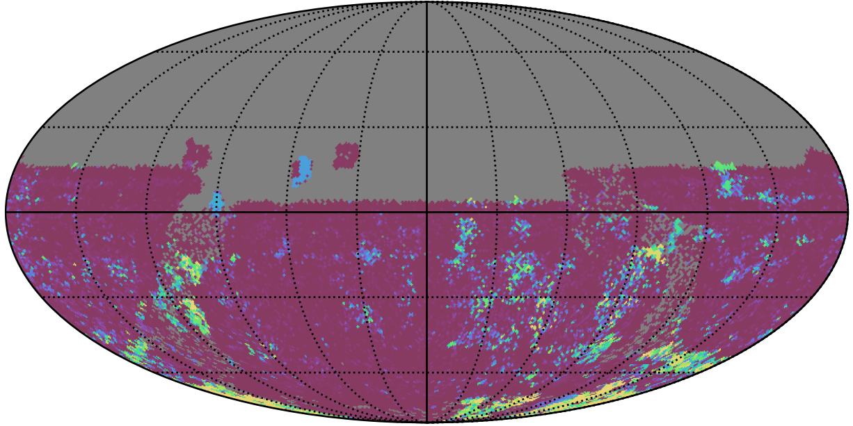
too_elab_heavy_r32_d2_ugrizy_v3.4_10yrs All sky u band: 75th Percentile Intranight Timespan
