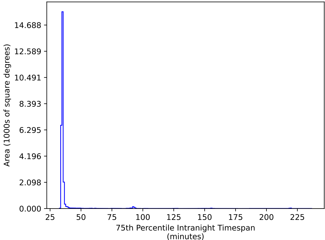
too_elab_heavy_r32_d2_ugrizy_v3.4_10yrs All sky ri bands: 75th Percentile Intranight Timespan
