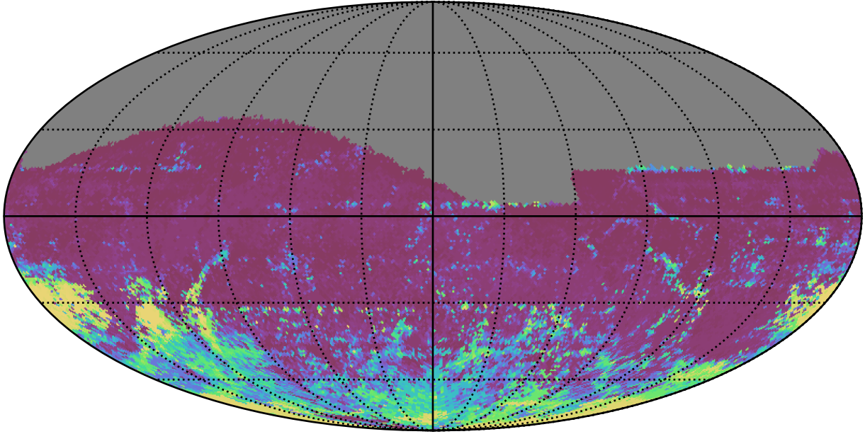
too_elab_heavy_r32_d2_ugrizy_v3.4_10yrs All sky r band: 75th Percentile Intranight Timespan
