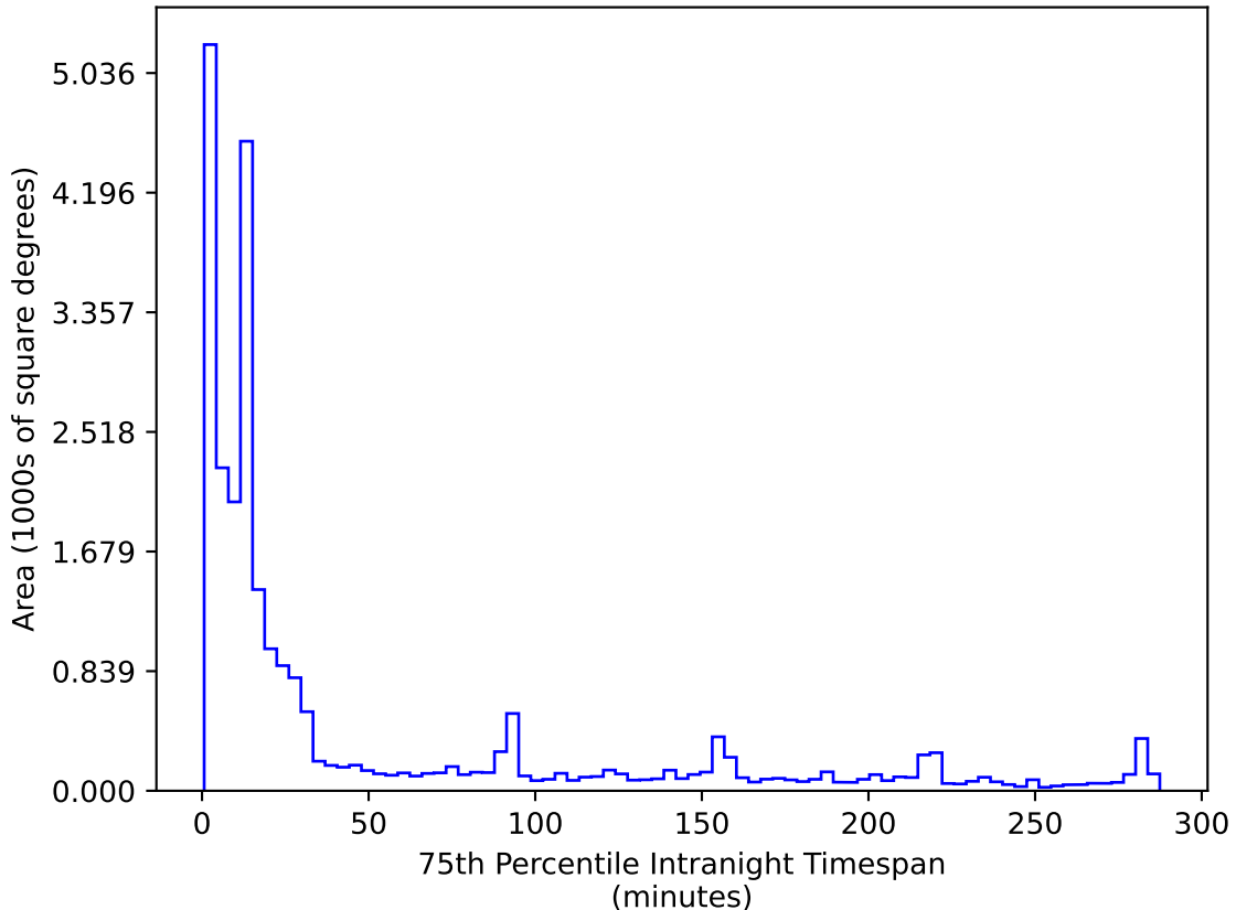
too_elab_heavy_r32_d2_ugrizy_v3.4_10yrs All sky r band: 75th Percentile Intranight Timespan
