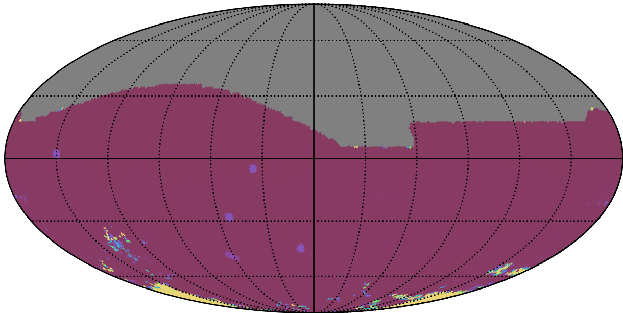
too_elab_heavy_r32_d2_ugrizy_v3.4_10yrs All sky iz bands: 75th Percentile Intranight Timespan
