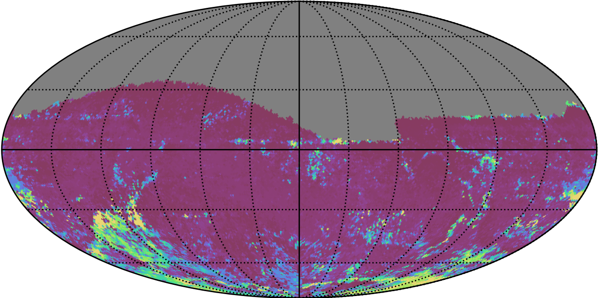
too_elab_heavy_r32_d2_ugrizy_v3.4_10yrs All sky i band: 75th Percentile Intranight Timespan
