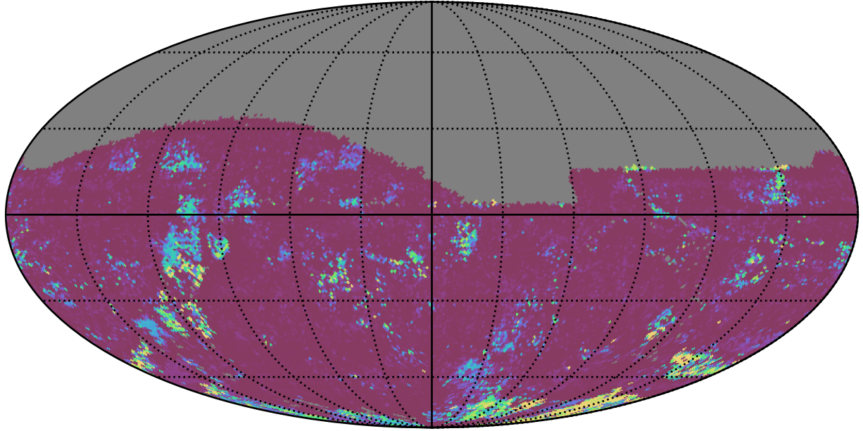
too_elab_heavy_r32_d2_ugrizy_v3.4_10yrs All sky g band: 75th Percentile Intranight Timespan
