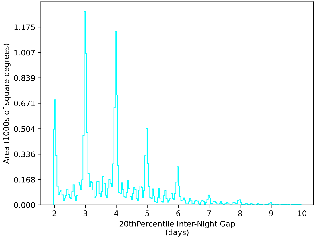
too_elab_heavy_r32_d2_ugrizy_v3.4_10yrs WFD u band: 20thPercentile Inter-Night Gap
