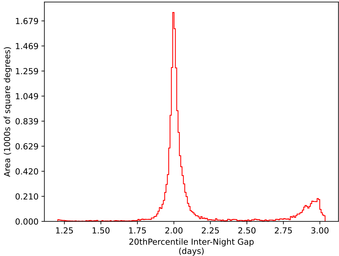
too_elab_heavy_r32_d2_ugrizy_v3.4_10yrs WFD i band: 20thPercentile Inter-Night Gap
