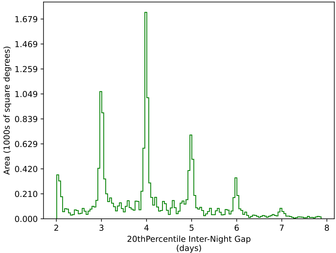
too_elab_heavy_r32_d2_ugrizy_v3.4_10yrs WFD g band: 20thPercentile Inter-Night Gap
