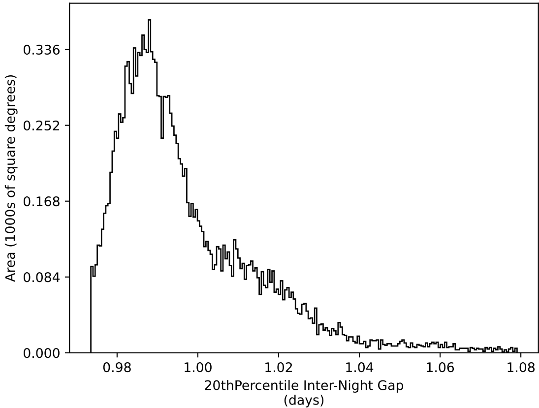
too_elab_heavy_r32_d2_ugrizy_v3.4_10yrs WFD all bands: 20thPercentile Inter-Night Gap
