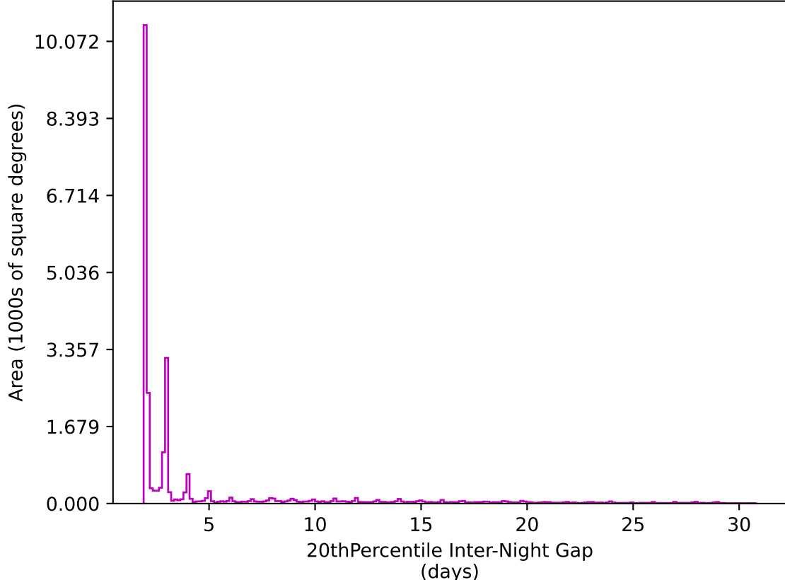
too_elab_heavy_r32_d2_ugrizy_v3.4_10yrs All sky z band: 20thPercentile Inter-Night Gap
