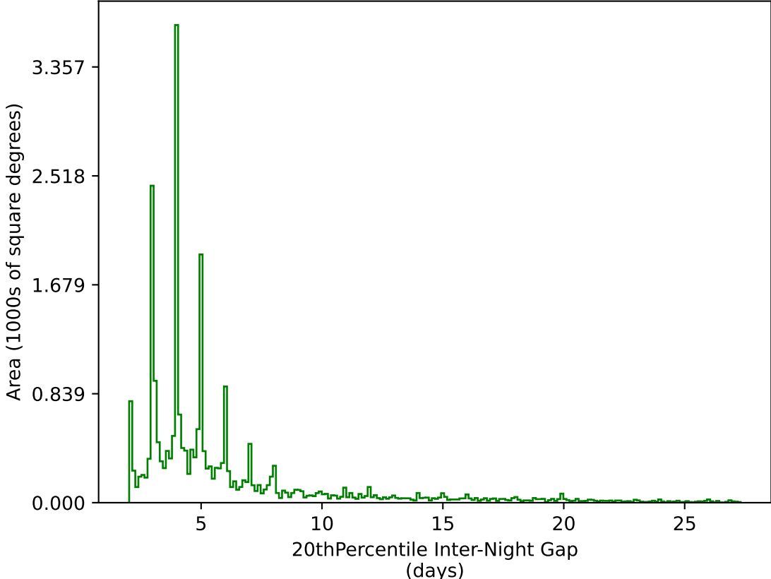
too_elab_heavy_r32_d2_ugrizy_v3.4_10yrs All sky g band: 20thPercentile Inter-Night Gap
