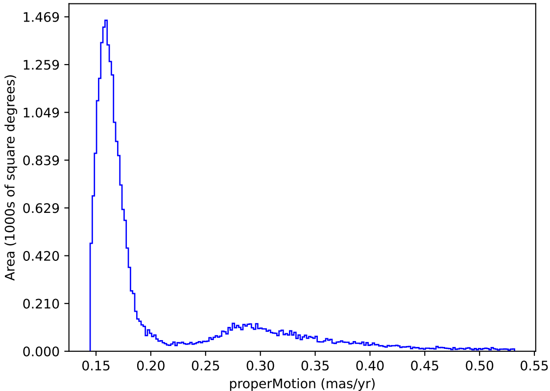
too_elab_heavy_r32_d2_ugrizy_v3.4_10yrs : properMotion
