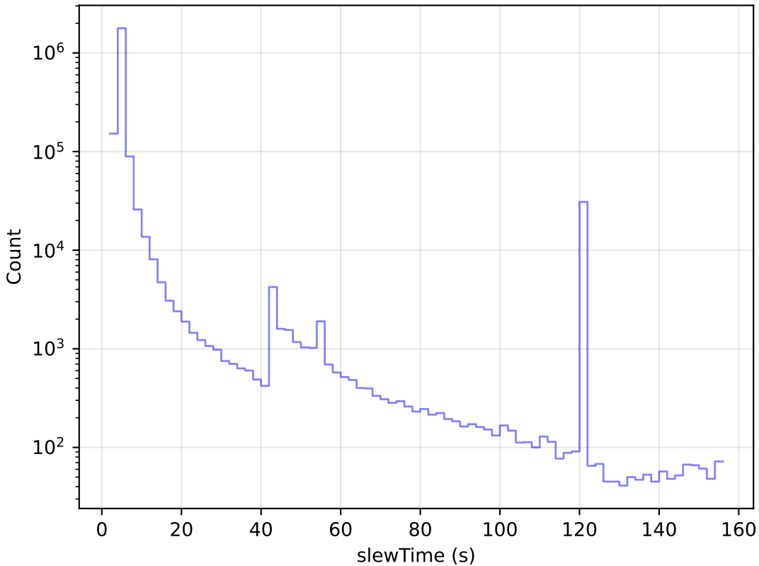
too_elab_heavy_r32_d2_ugrizy_v3.4_10yrs All visits: Slew Time Histogram
