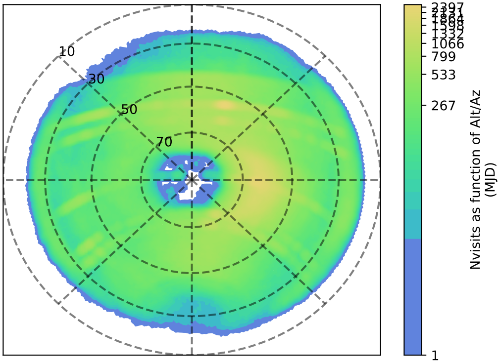
too_elab_heavy_r32_d2_ugrizy_v3.4_10yrs z: Nvisits as function of Alt/Az
