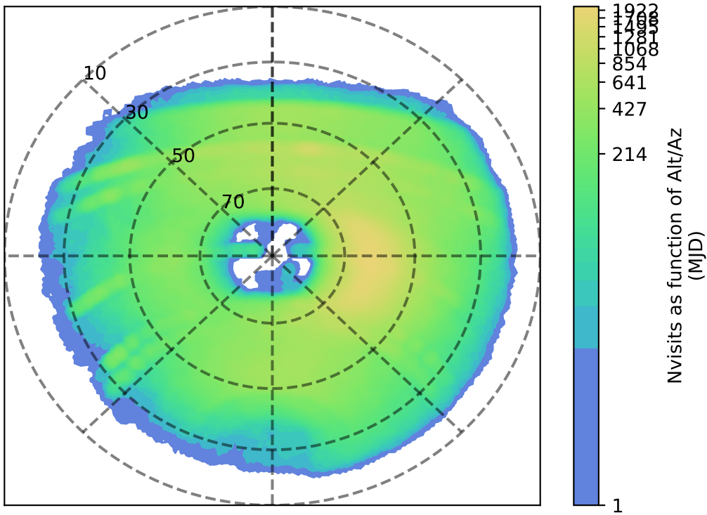
too_elab_heavy_r32_d2_ugrizy_v3.4_10yrs y: Nvisits as function of Alt/Az
