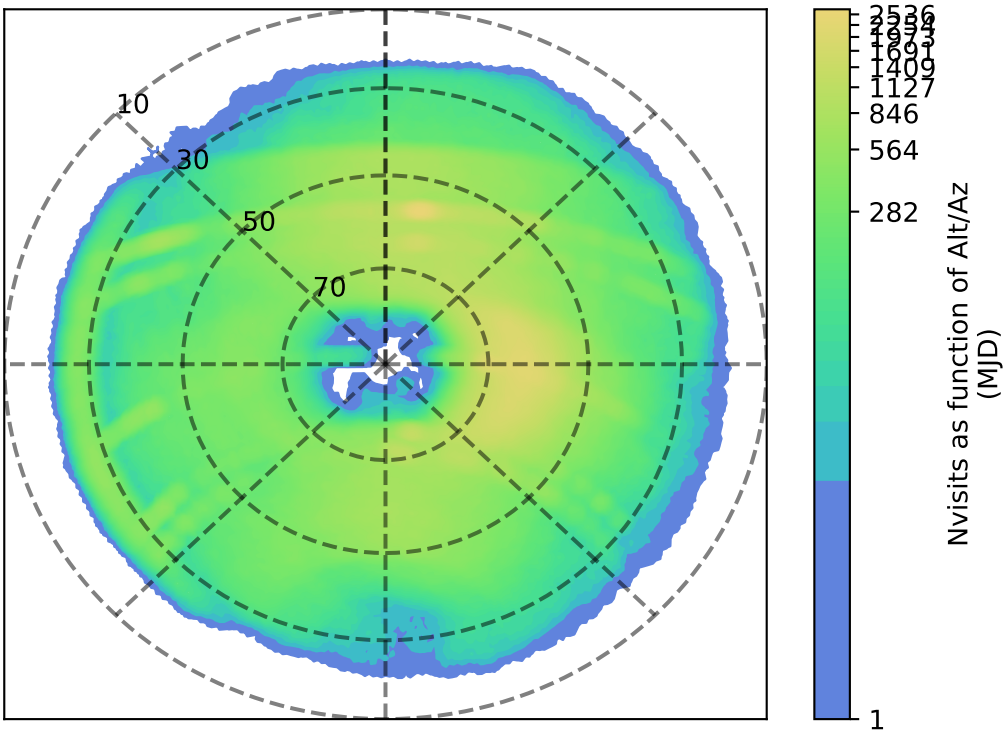
too_elab_heavy_r32_d2_ugrizy_v3.4_10yrs r: Nvisits as function of Alt/Az
