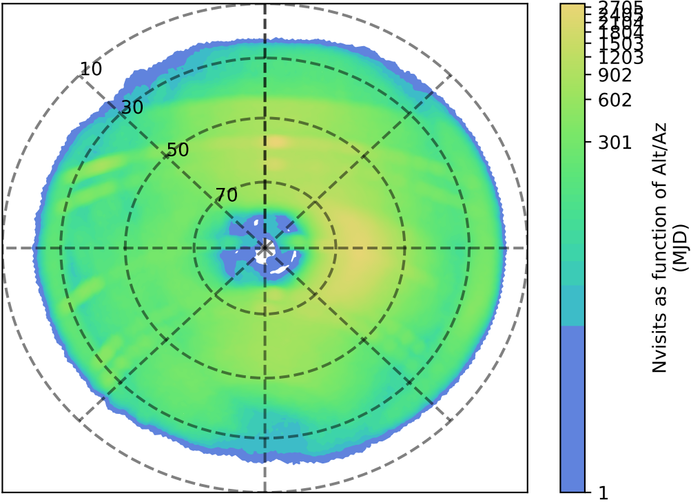
too_elab_heavy_r32_d2_ugrizy_v3.4_10yrs i: Nvisits as function of Alt/Az
