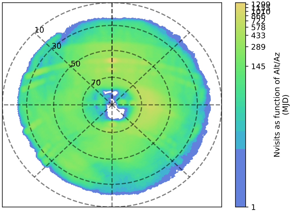
too_elab_heavy_r32_d2_ugrizy_v3.4_10yrs g: Nvisits as function of Alt/Az
