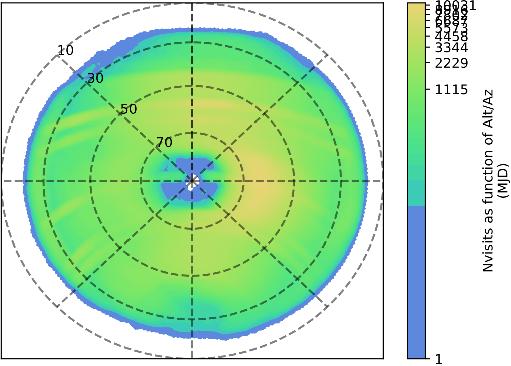
too_elab_heavy_r32_d2_ugrizy_v3.4_10yrs : Nvisits as function of Alt/Az
