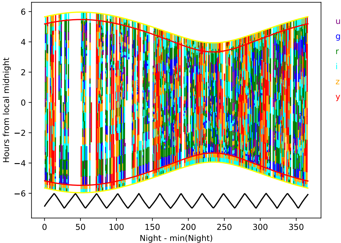
too_elab_heavy_r32_d2_ugrizy_v3.4_10yrs year 8-9: Hourglass
