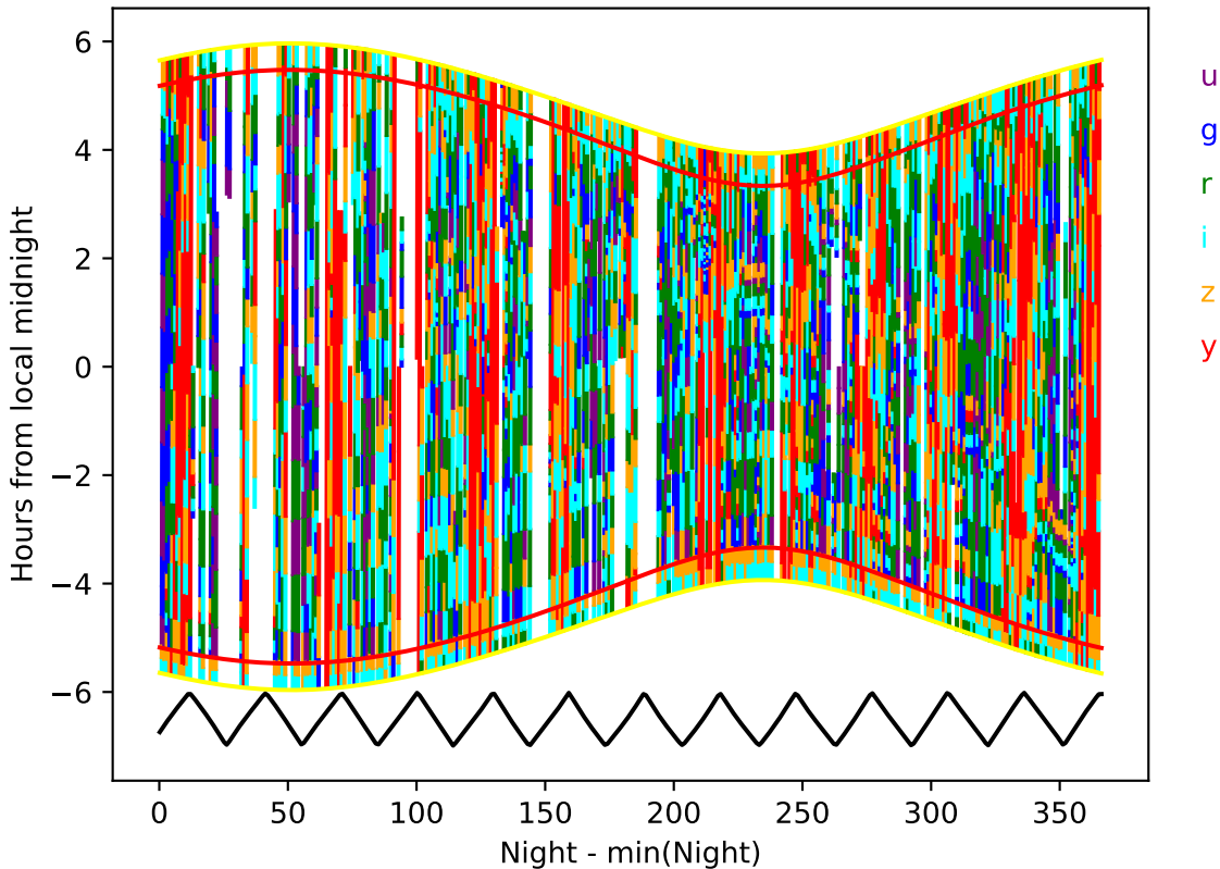
too_elab_heavy_r32_d2_ugrizy_v3.4_10yrs year 0-1: Hourglass
