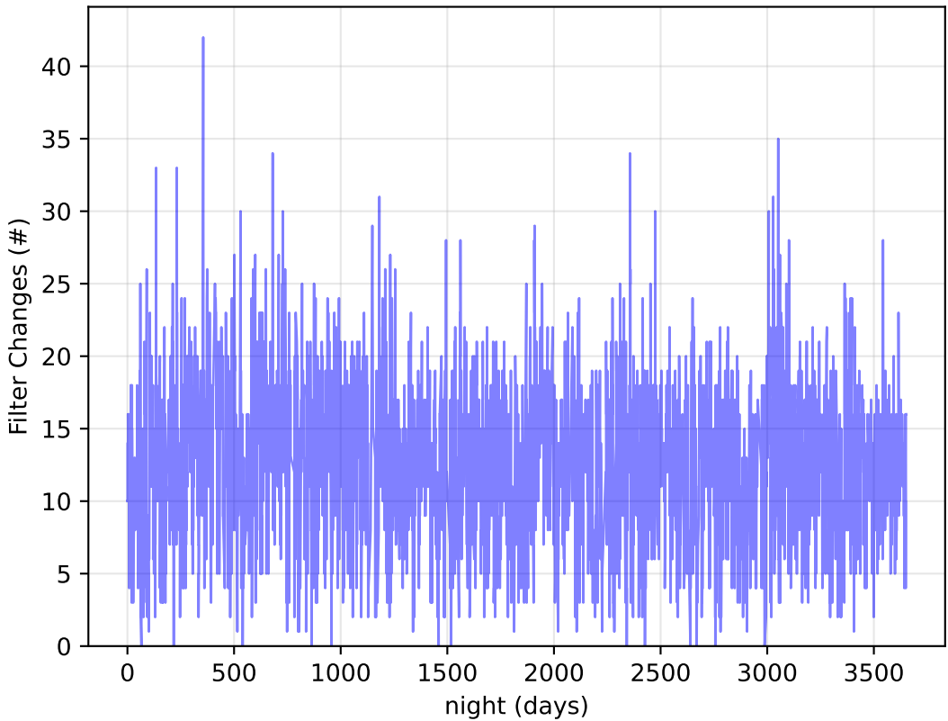
too_elab_heavy_r32_d2_ugrizy_v3.4_10yrs : Filter Changes
