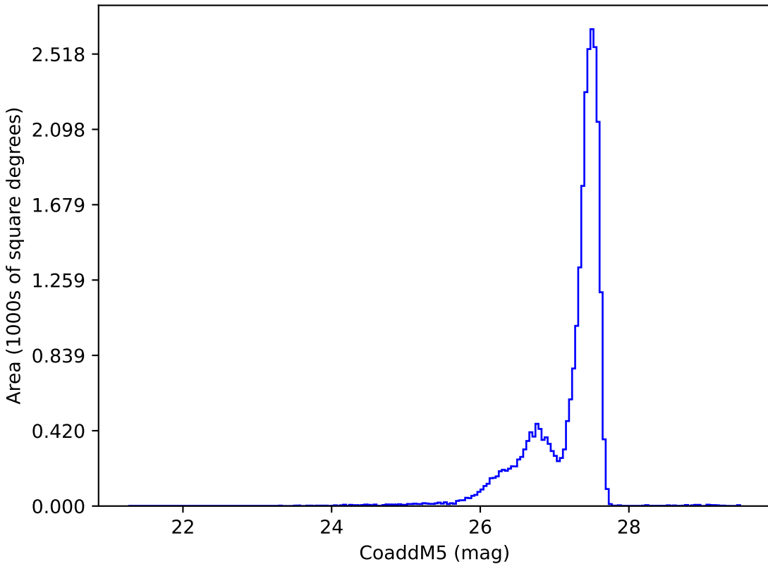
too_elab_heavy_r32_d2_ugrizy_v3.4_10yrs : CoaddM5
