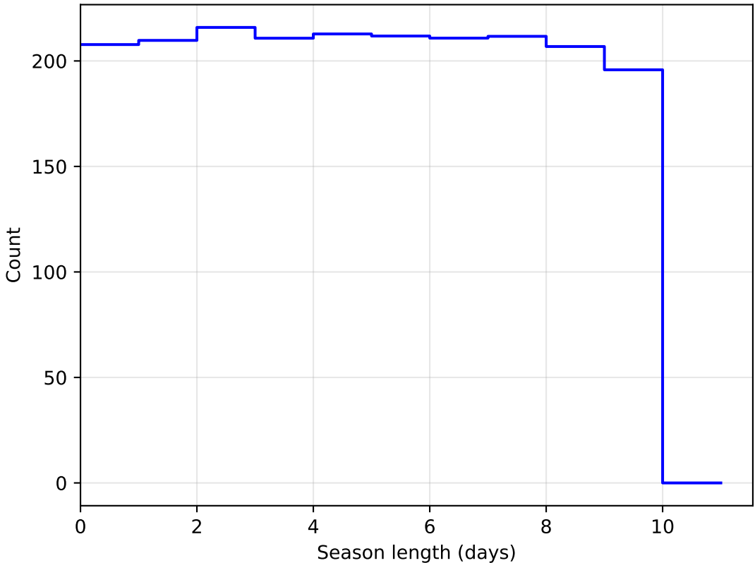
too_elab_heavy_r32_d2_ugrizy_v3.4_10yrs DD:EDFS all bands: SeasonLength
