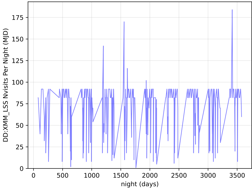
too_elab_heavy_r32_d2_ugrizy_v3.4_10yrs all bands: DD:XMM_LSS Nvisits Per Night
