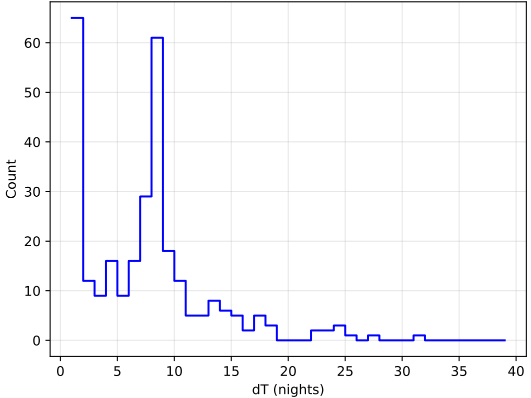
too_elab_heavy_r32_d2_ugrizy_v3.4_10yrs all bands: DD:XMM_LSS Delta Nights Histogram
