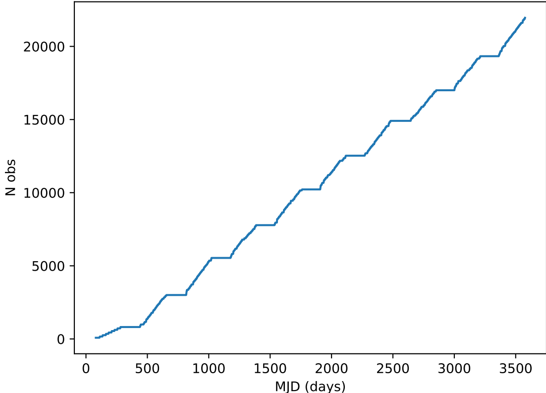
too_elab_heavy_r32_d2_ugrizy_v3.4_10yrs all bands: DD:XMM_LSS Cumulative NVisits
