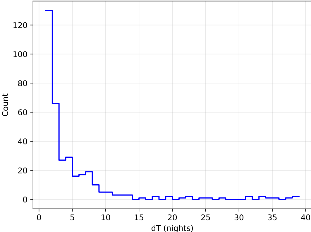
too_elab_heavy_r32_d2_ugrizy_v3.4_10yrs all bands: DD:WFD Delta Nights Histogram
