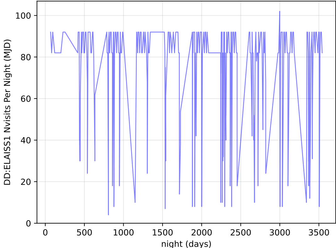
too_elab_heavy_r32_d2_ugrizy_v3.4_10yrs all bands: DD:ELAISS1 Nvisits Per Night
