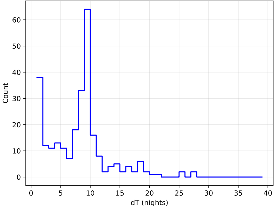
too_elab_heavy_r32_d2_ugrizy_v3.4_10yrs all bands: DD:ELAISS1 Delta Nights Histogram
