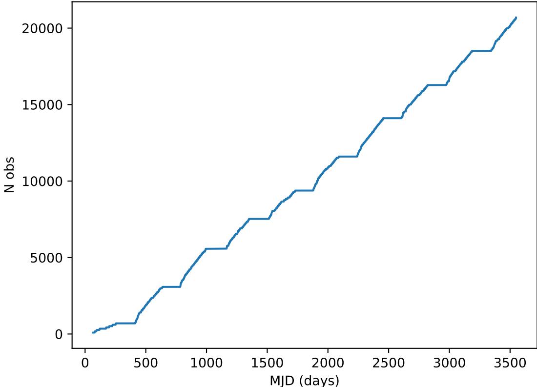
too_elab_heavy_r32_d2_ugrizy_v3.4_10yrs all bands: DD:ELAISS1 Cumulative NVisits
