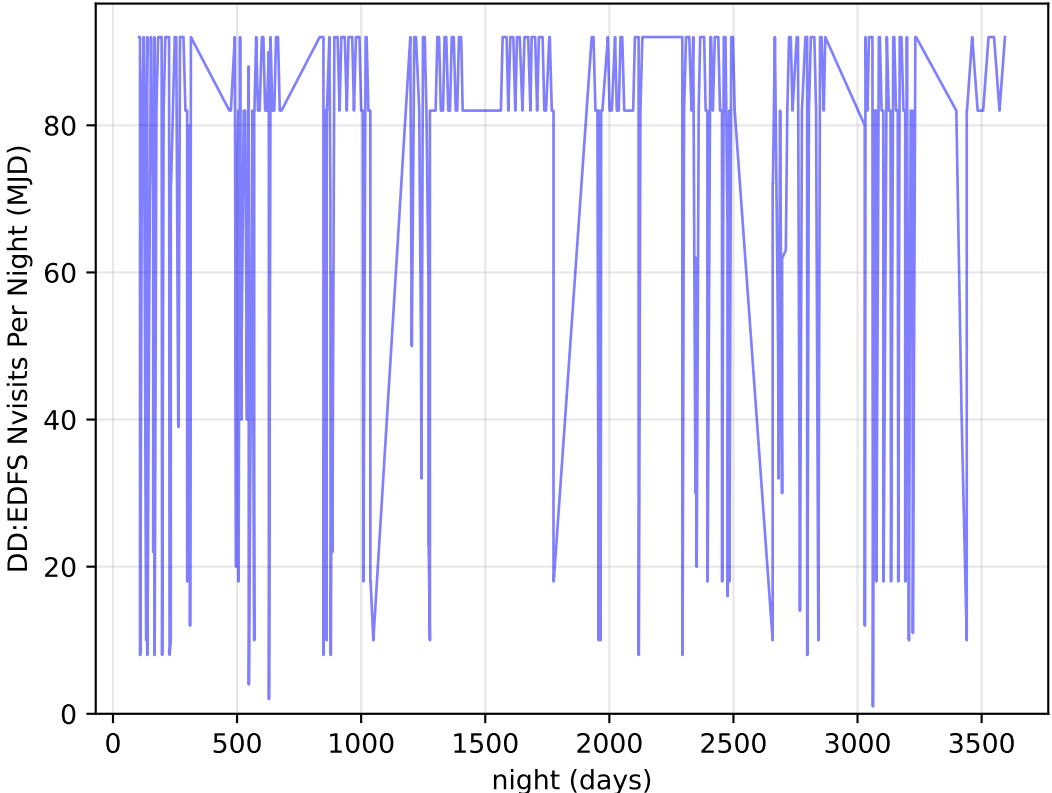
too_elab_heavy_r32_d2_ugrizy_v3.4_10yrs all bands: DD:EDFS Nvisits Per Night
