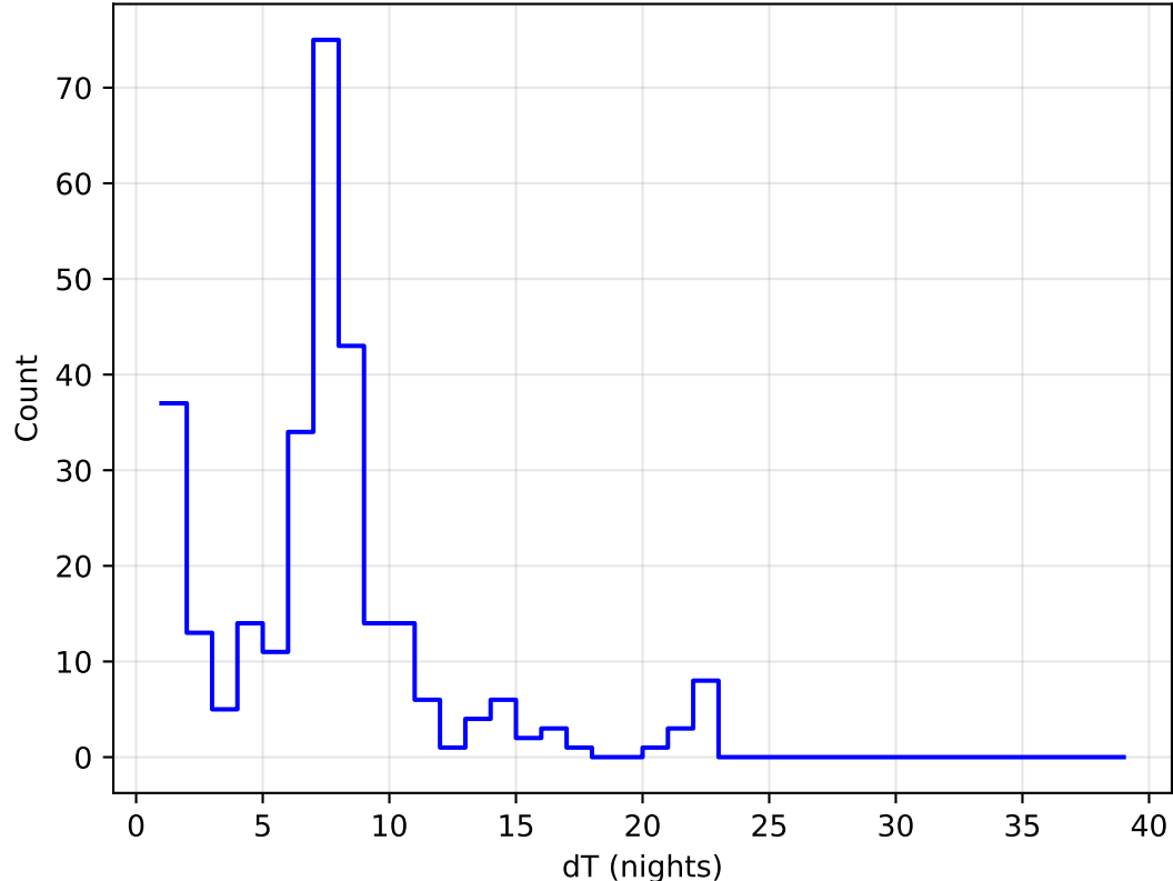
too_elab_heavy_r32_d2_ugrizy_v3.4_10yrs all bands: DD:EDFS Delta Nights Histogram
