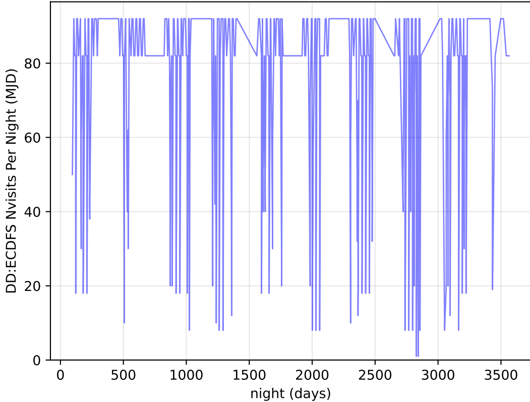
too_elab_heavy_r32_d2_ugrizy_v3.4_10yrs all bands: DD:ECDFS Nvisits Per Night
