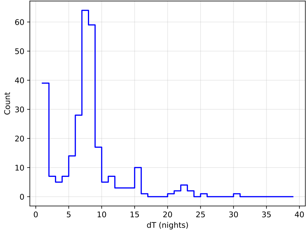
too_elab_heavy_r32_d2_ugrizy_v3.4_10yrs all bands: DD:ECDFS Delta Nights Histogram
