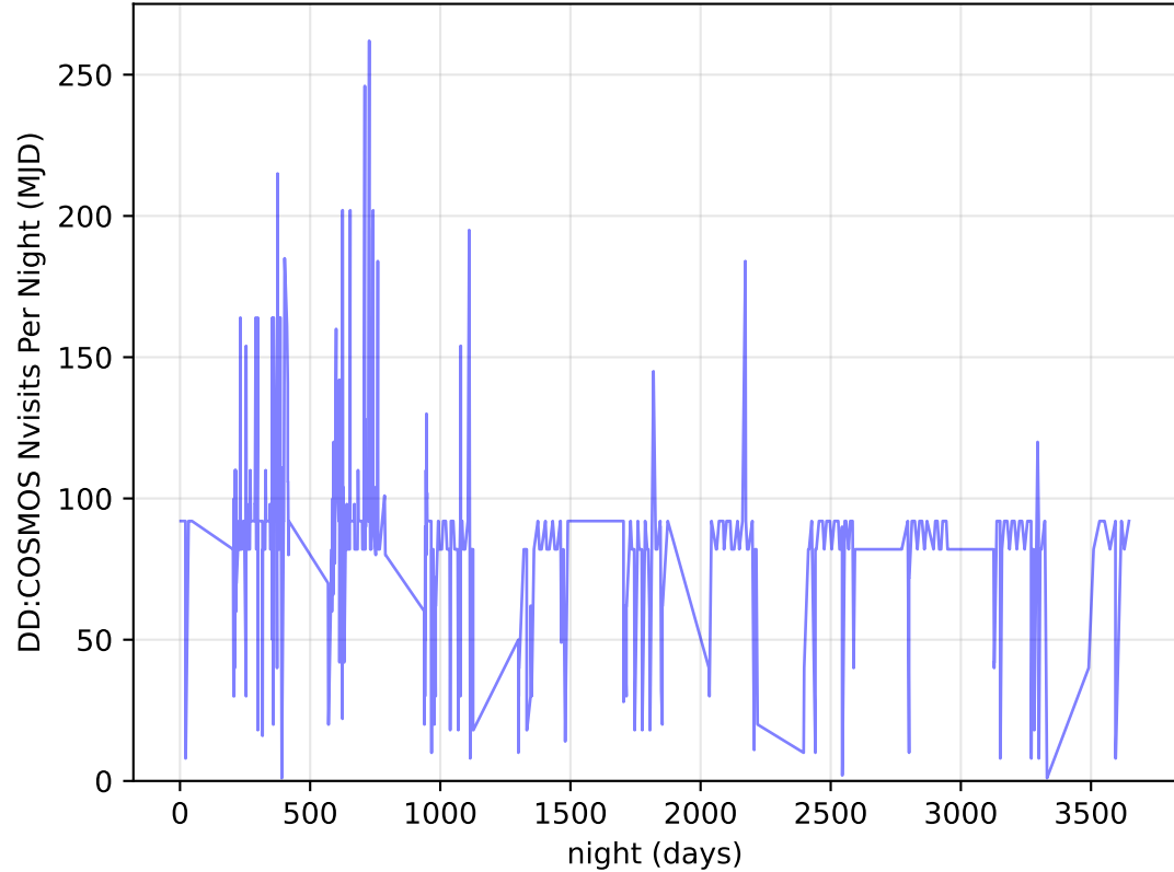
too_elab_heavy_r32_d2_ugrizy_v3.4_10yrs all bands: DD: COSMOS Nvisits Per Night
