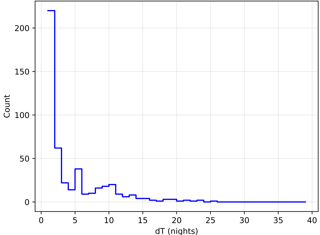
too_elab_heavy_r32_d2_ugrizy_v3.4_10yrs all bands: DD: COSMOS Delta Nights Histogram
