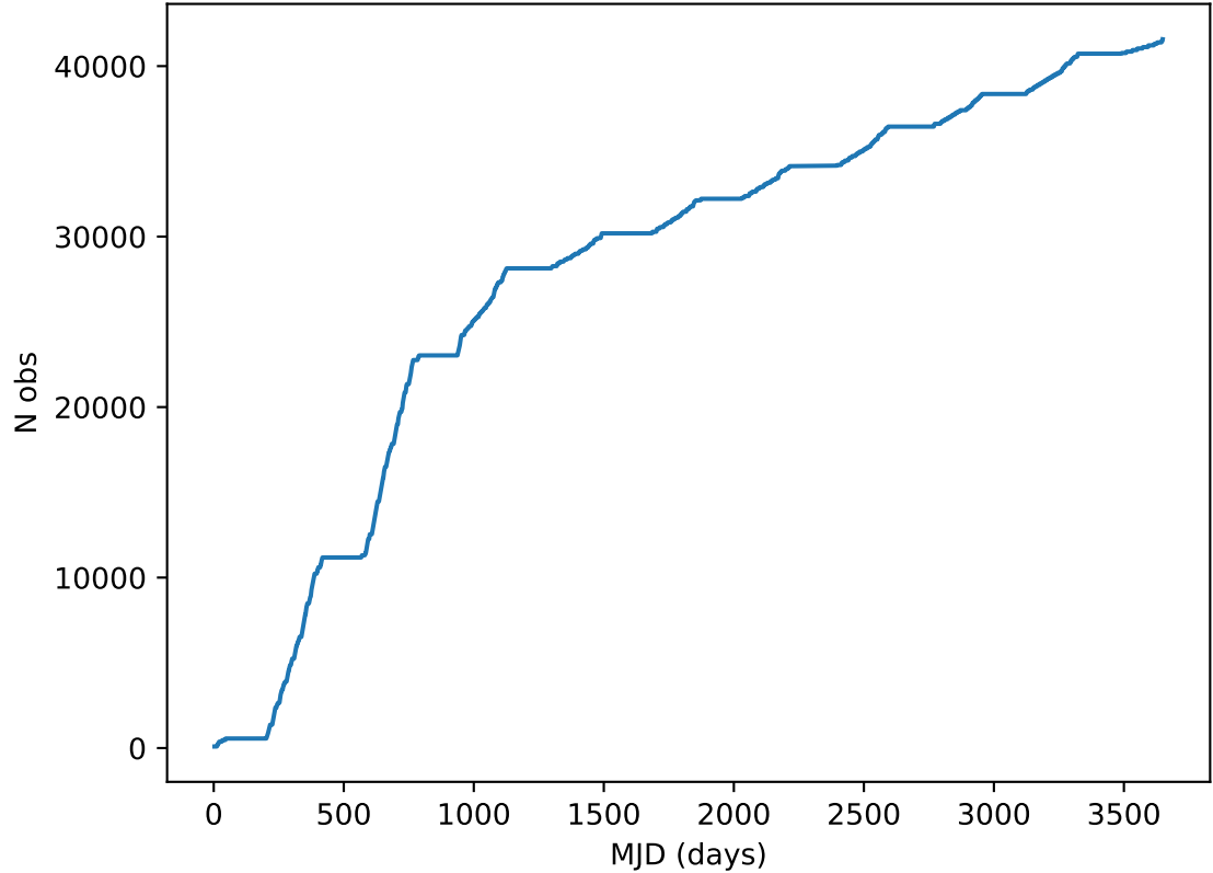
too_elab_heavy_r32_d2_ugrizy_v3.4_10yrs all bands: DD: COSMOS Cumulative NVisits
