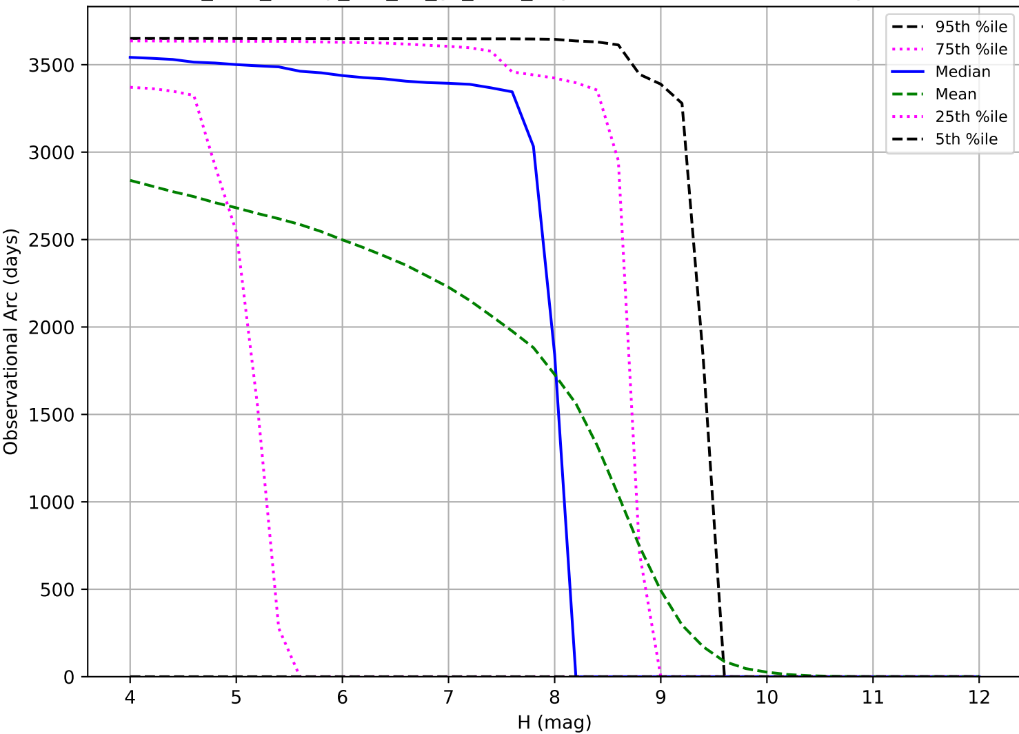
too_elab_heavy_r32_d2_gz_v3.4_10yrs: Observational Arc Length TNO
