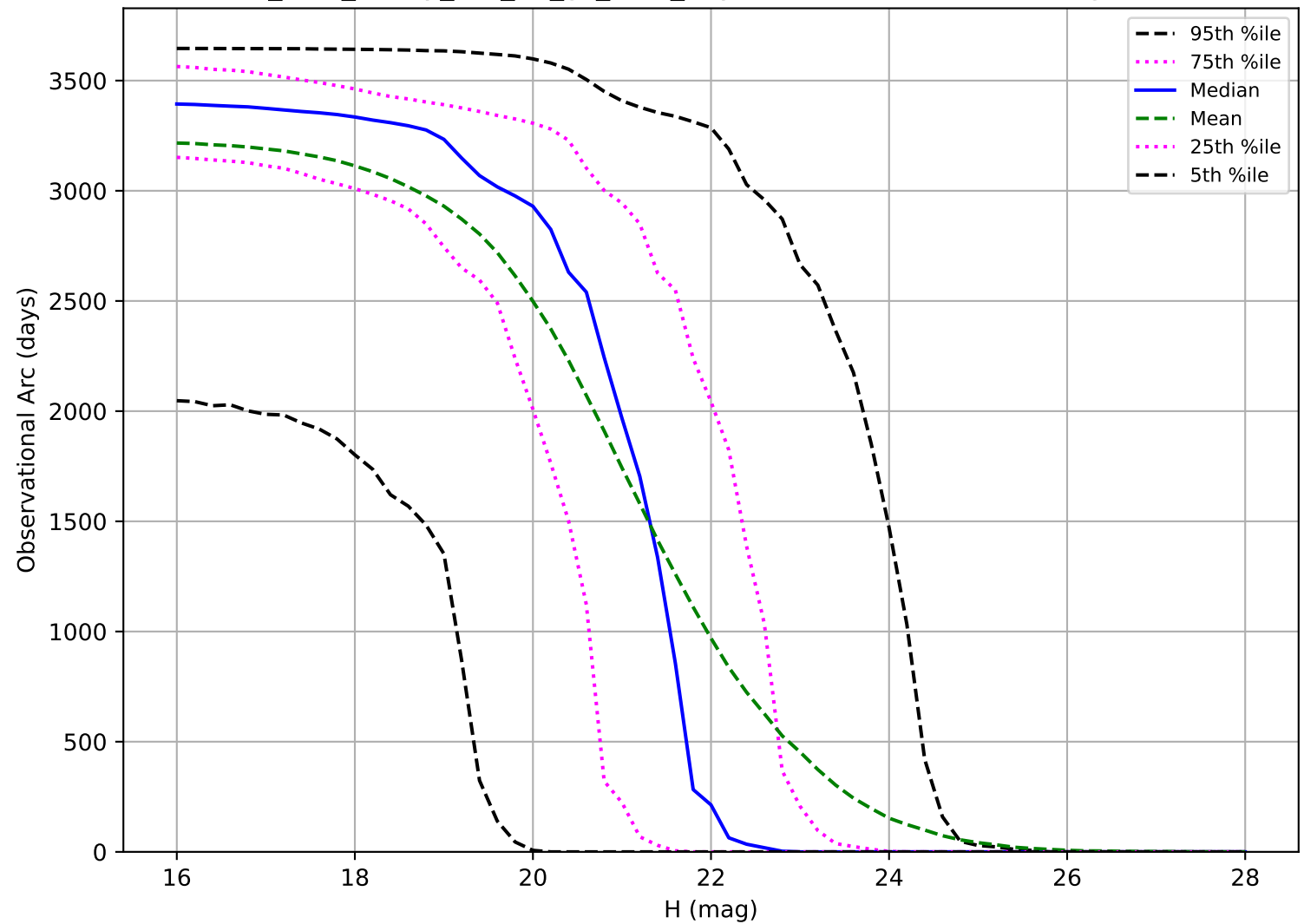
too_elab_heavy_r32_d2_gz_v3.4_10yrs: Observational Arc Length PHA
