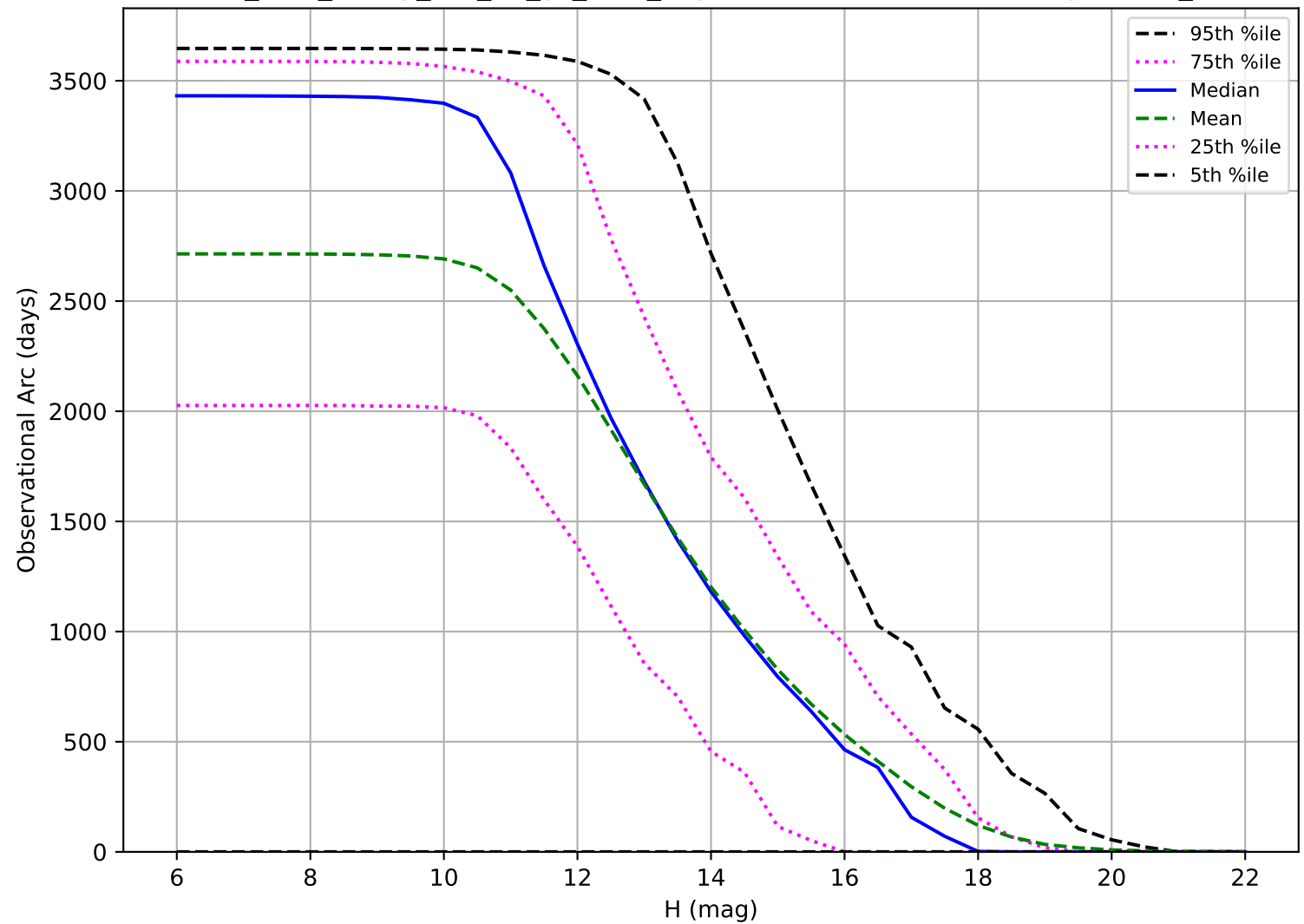
too_elab_heavy_r32_d2_gz_v3.4_10yrs: Observational Arc Length OCC_r5
