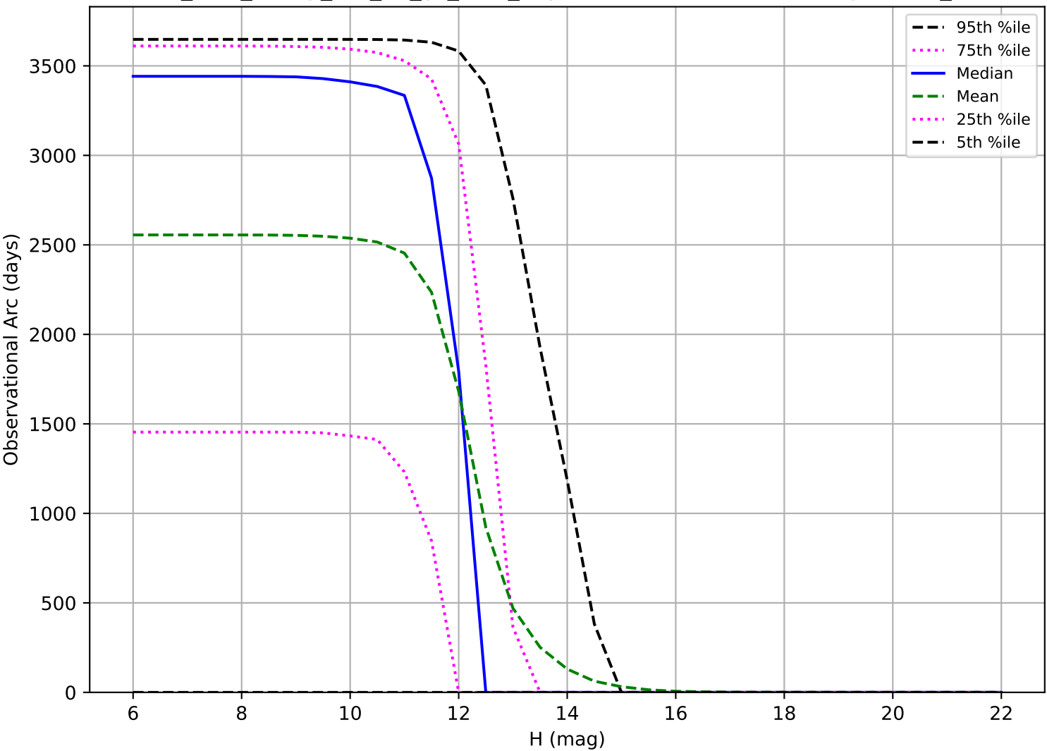
too_elab_heavy_r32_d2_gz_v3.4_10yrs: Observational Arc Length OCC_r20
