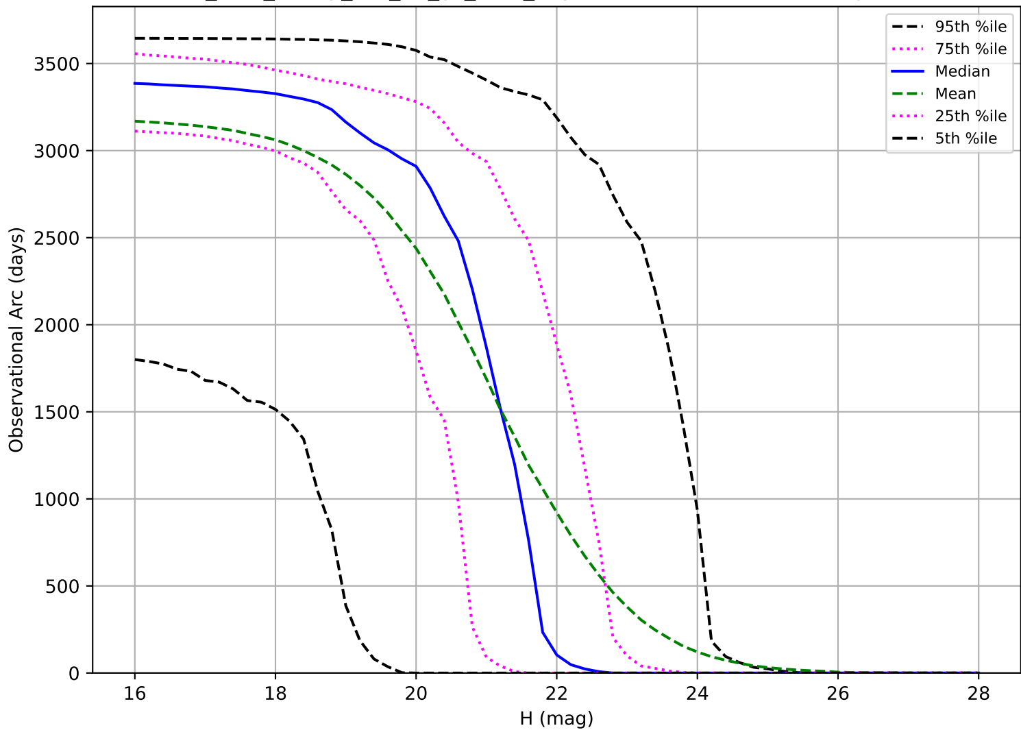
too_elab_heavy_r32_d2_gz_v3.4_10yrs: Observational Arc Length NEO
