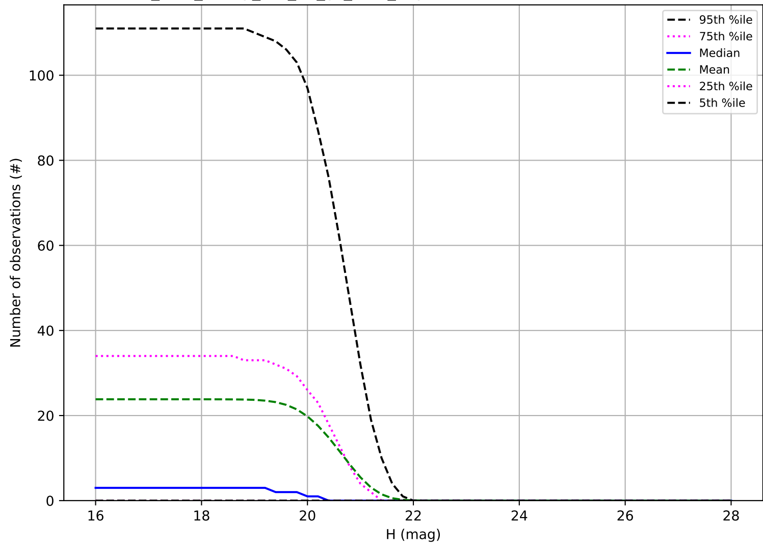
too_elab_heavy_r32_d2_gz_v3.4_10yrs: Number of observations Vatira
