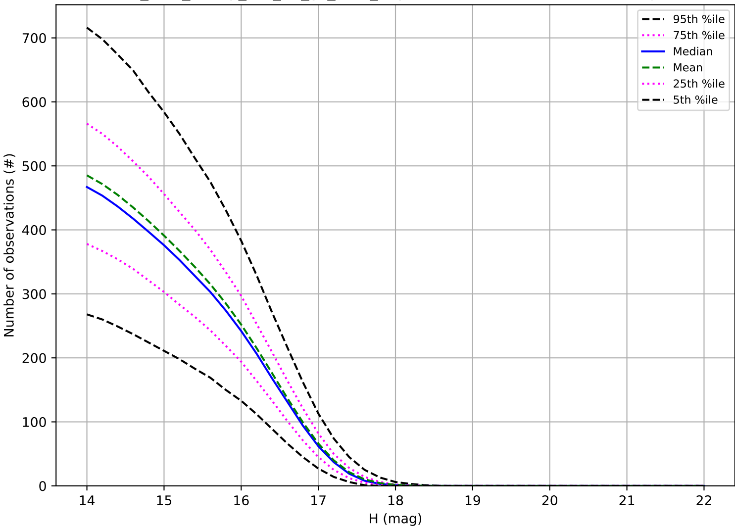
too_elab_heavy_r32_d2_gz_v3.4_10yrs: Number of observations Trojan
