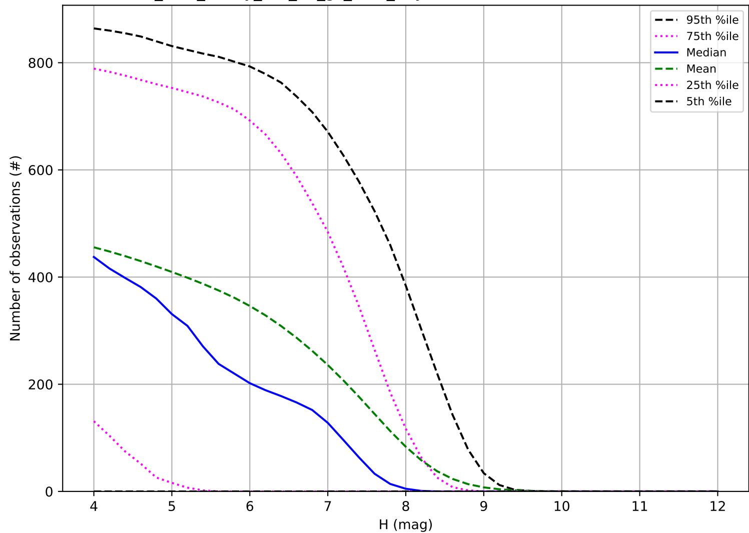
too_elab_heavy_r32_d2_gz_v3.4_10yrs: Number of observations TNO
