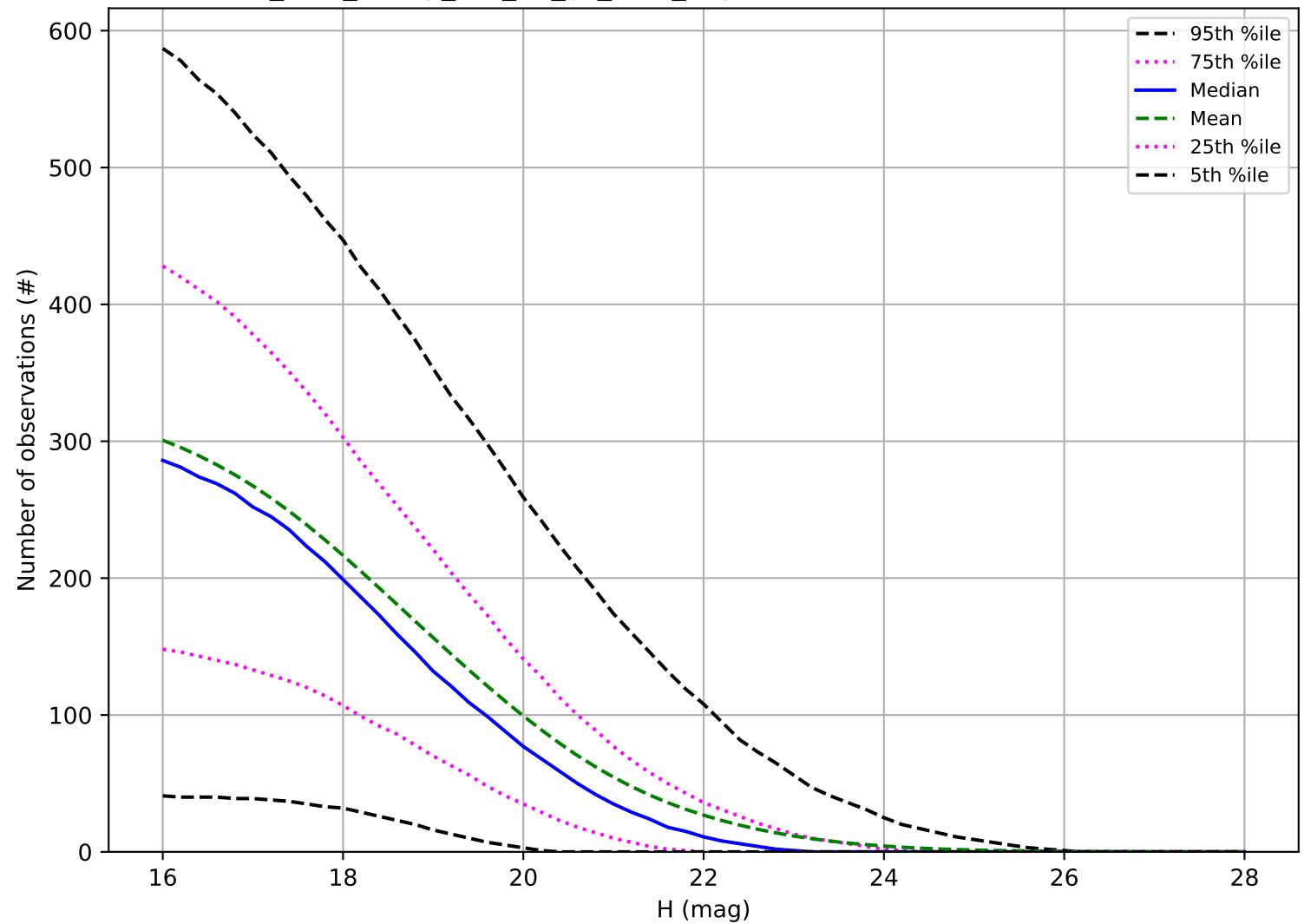
too_elab_heavy_r32_d2_gz_v3.4_10yrs: Number of observations PHA
