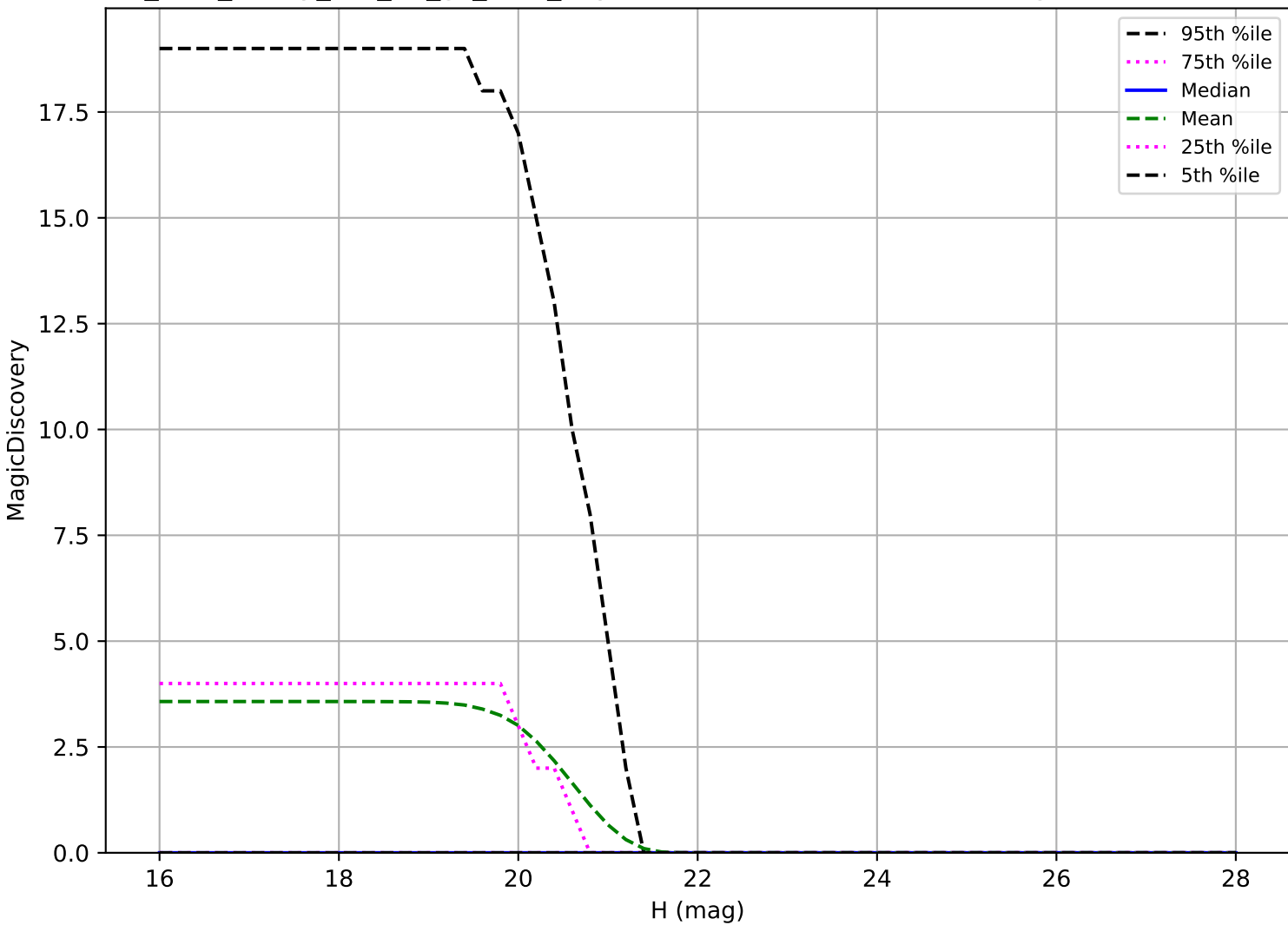
too_elab_heavy_r32_d2_gz_v3.4_10yrs: Vatira 6 detections in 60 nights detection loss
